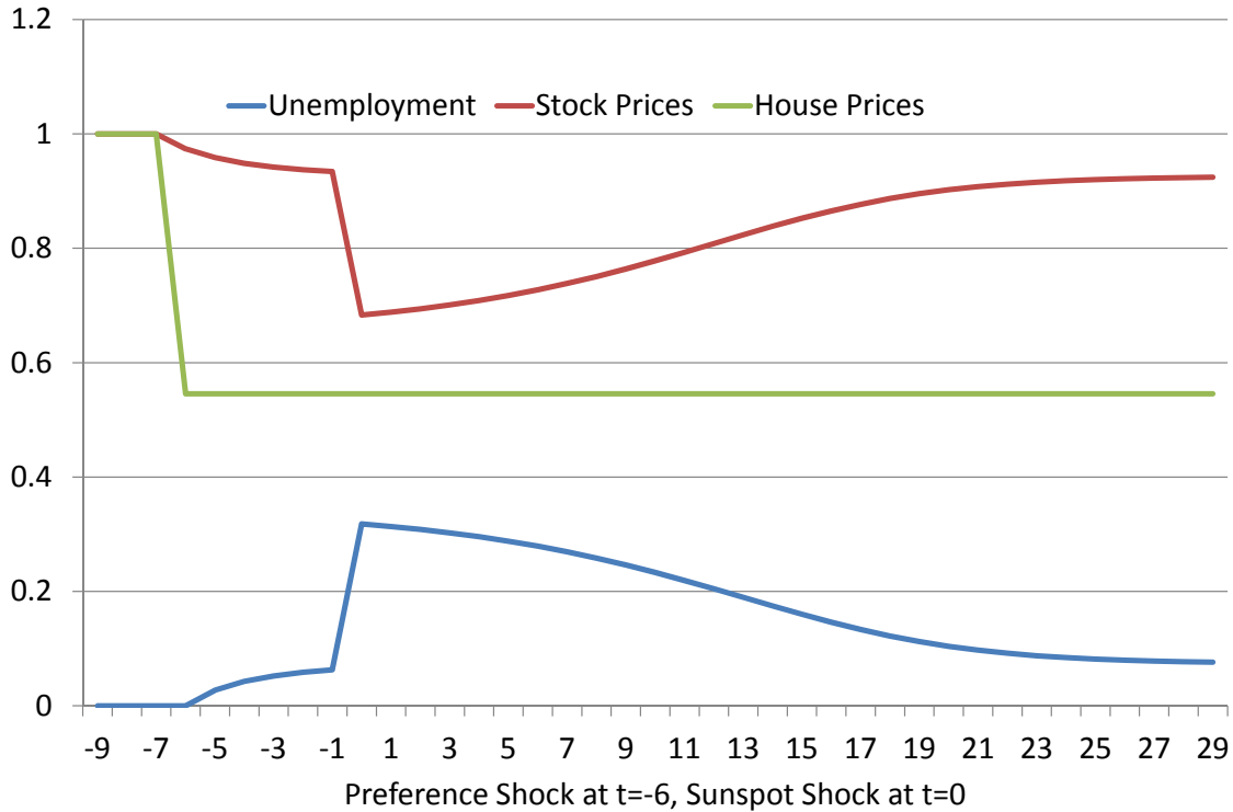
Figure 11: Model's prediction
